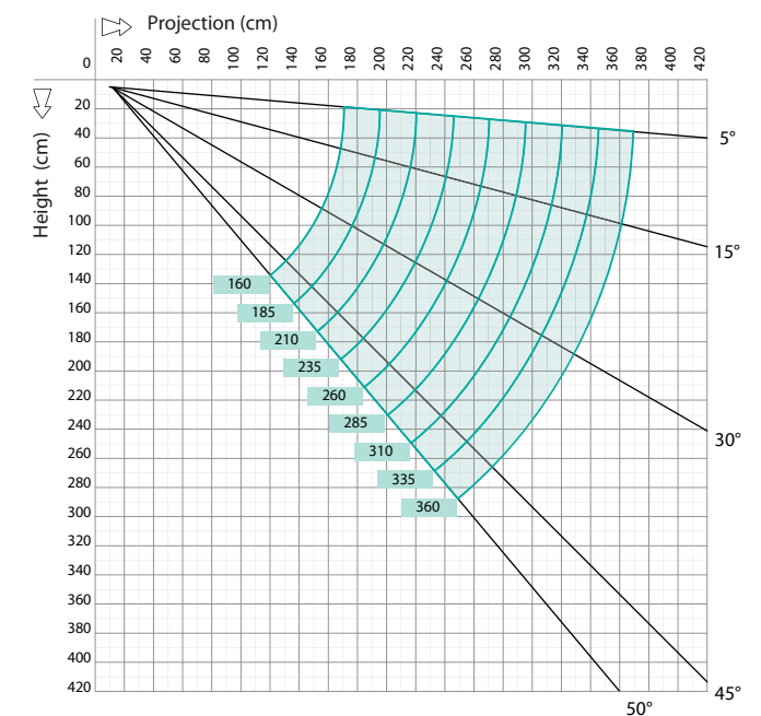
Wall covering diagram
