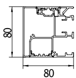
Profiles dimensions (mm)
