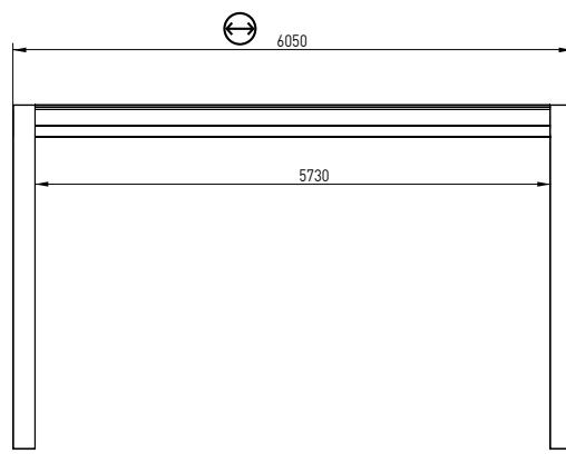
General technical plan (mm)
