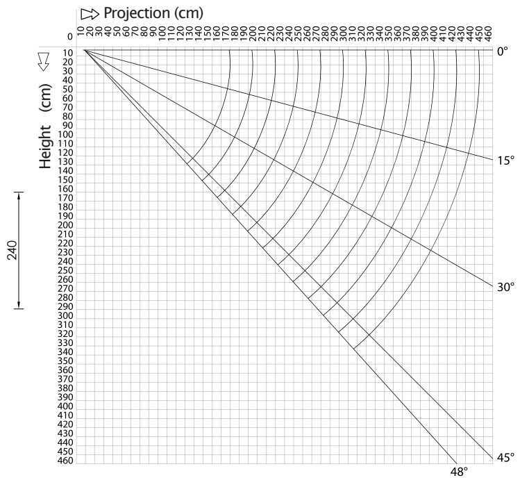
Ceiling covering diagram
